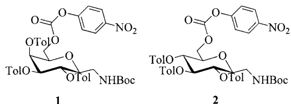
Figure 1. The Glycosylmethylamine carbonates 1 and 2 used as building blocks.
