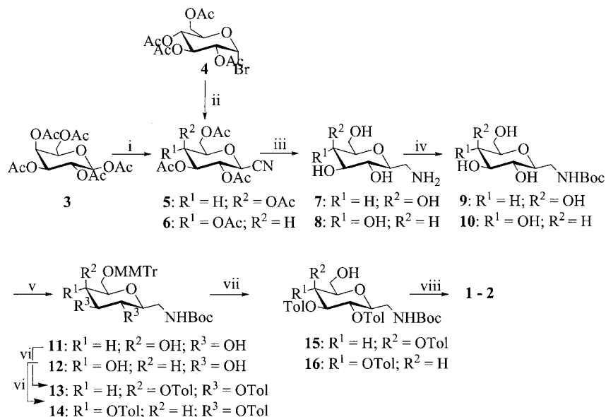
Scheme 1. Conditions: (i) TMSCN, BF_3 \cdot Et_2O , MeNO_2 , 74%; (ii) Hg(CN)_2 , melt, 85 °C, 41%; (iii) LiAlH_4 , THF, (iv) Boc_2O , 2 mol L -1 NaOH, MeCN, H 2 O, 9: 53% (from 5), 10: 14% (from 6), (v) MMTTrCl, NEt_3 , DMAP, DMF, 11: 69%, 12: 77%; (vi) p -MeBzCl, pyridine, 13: 79%, 14: 52%; (vii) I 2 , MeOH, CH_2Cl_2 , 15: 98%, 16: 97%; (viii) p -nitrophenyl chloroformate, DMAP, pyridine, 1: 52%, 2: 66%.
