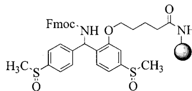
Figure 2. An aminomethyl-polystyrene support derivatized with a SCAL linker.
