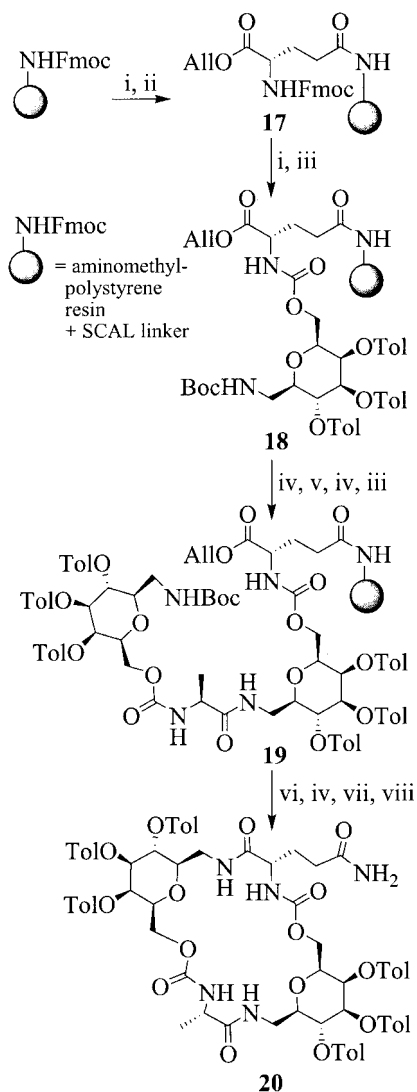
Scheme 2. Conditions: (i) Piperidine, DMF; (ii) Fmoc-Glu-OAll, PyAOP, DIEA, DMF; (iii) 1 , DIEA, HOBt, NMP; (iv) TFA, CH 2 Cl 2 ; (v) Boc-Ala-OH, PyAOP, DIEA, DMF; (vi) Pd(OAc) 2 , Bu 3 SnH, PPh 3 , AcOH, CH 2 Cl 2 ; (vii) PyBOP, DIEA, DMF; (viii) 0.1% HBr in AcOH, TFA, CH 2 Cl 2 .
