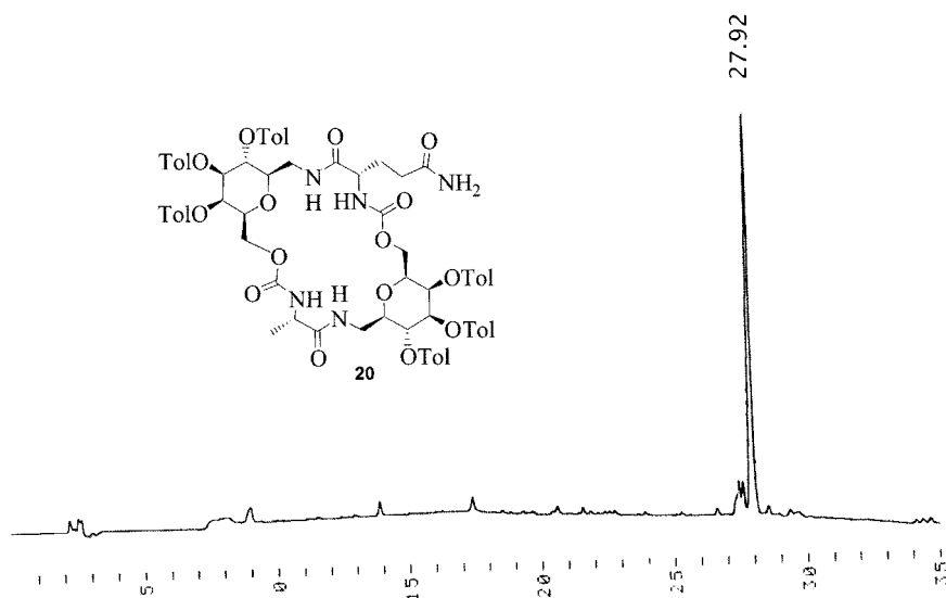
Figure 3. RP HPLC profile of crude 20 . Hypersil Hypurity C18 (150 × 4.6 mm, 5 μm), gradient from aqueous 0.1% TFA to acetonitrile in 30 min, flow 1.0 mL min -1 , detection at 215 nm.
